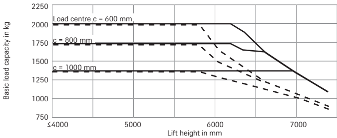
RX 70-20/600 600 triplex mast Single superelastic tyres
