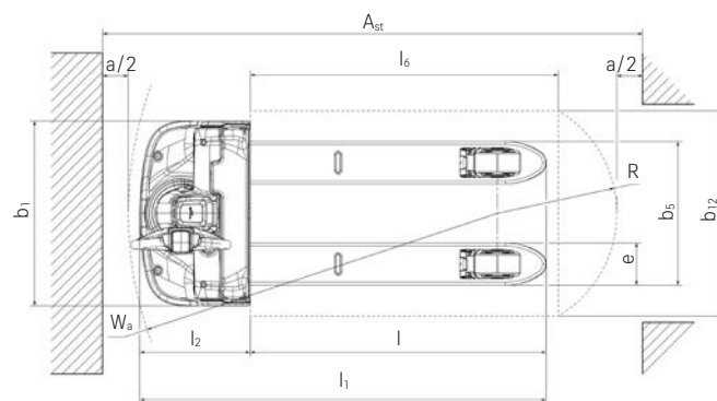
Top view EXH 16-20
