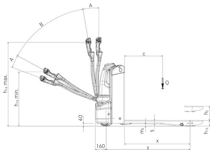
Side view EXH 16-20
